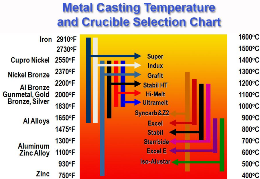
Fig. 4. A crucible must first support the range of metal temperatures it will encounter. But by offering products with overlapping temperature ranges, a crucible manufacturer is also able to provide a choice of crucibles with varying performance characteristics.
