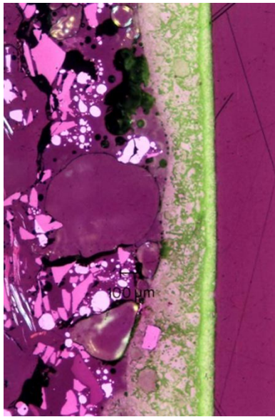
Fig. 6. This micro-section shows a fired-on refractory coating designed to resist metal and flux penetration of the crucible wall and to prevent metal, oxide and slag adherence to the internal surface of the crucible.
