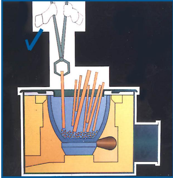
Fig. 5. Crucibles that provide impact resistance are often selected for furnaces that are manually charged with ingots and other solid materials.
